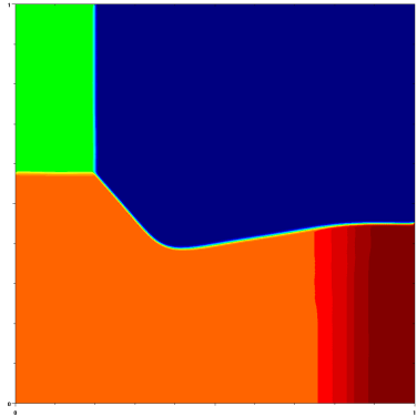
\mathbb{P}_1 FE, 3 \cdot 10^4 nodes
